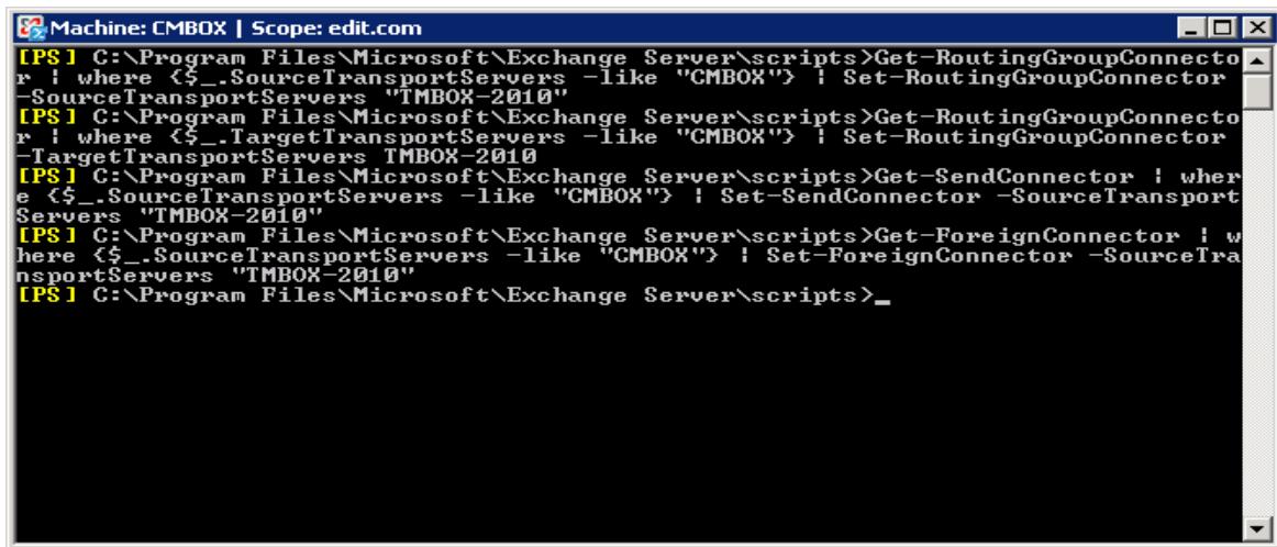
Figure 27: Moving the Routing Connectors from Exchange Server 2007 to Exchange Server 2010
