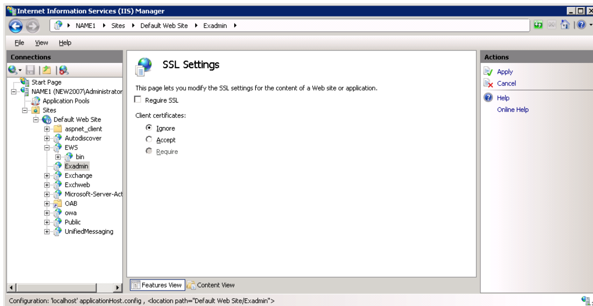
Figure 12: Disabling SSL in Exadmin
